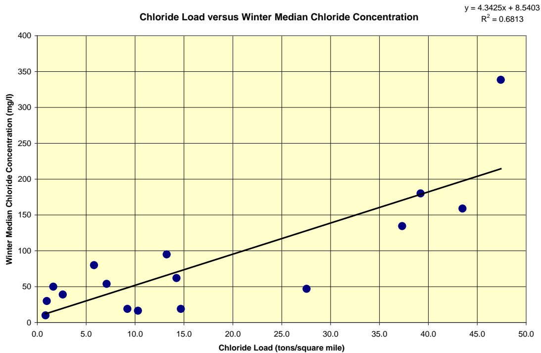
Figure 23. Relationship between road salt load and median winter stream chloride concentration (Wenck 2009)
