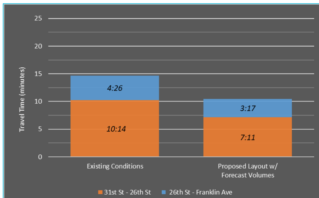
Figure 18. Northbound - Transit Vehicle Travel Time (PM Peak Hour)
