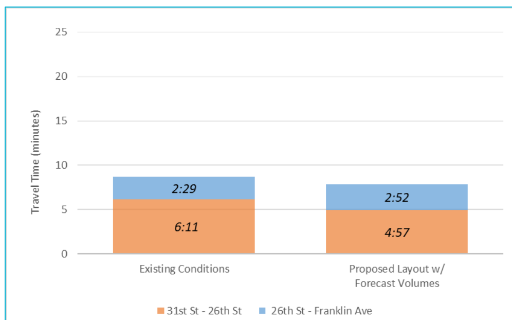
Figure 14. Northbound – Motor Vehicle Travel Time (PM Peak Hour)
