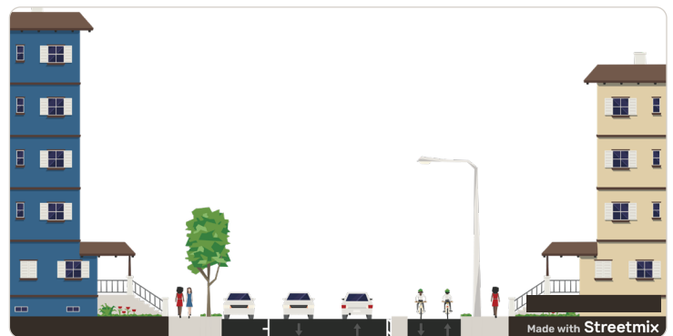
Figure 2: Proposed 40th St configuration with curb protection
